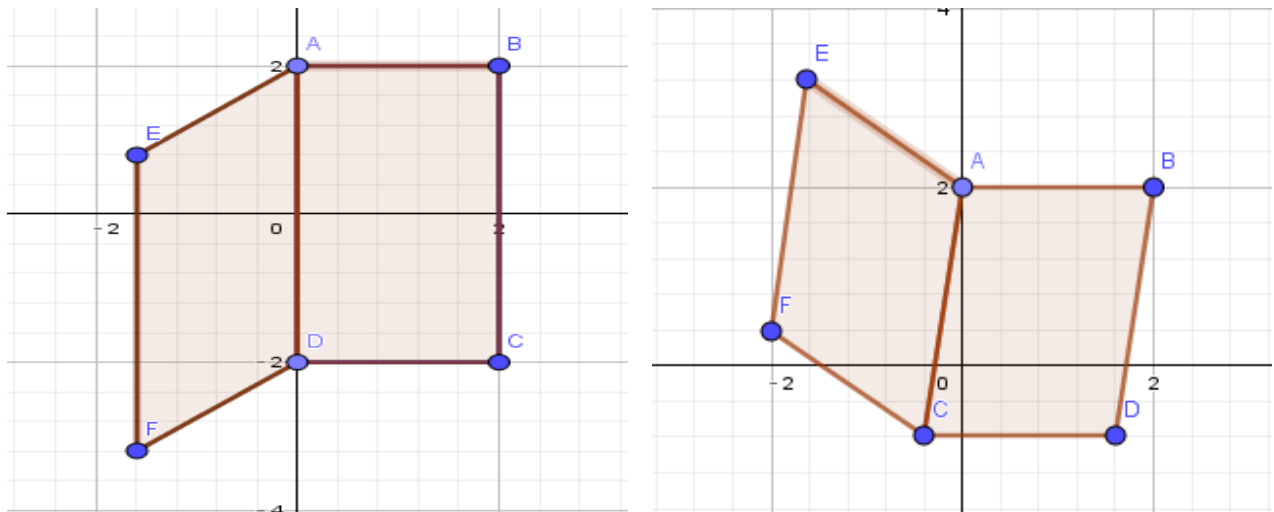
Figure-2. Examples of a straight line EF parallel to the plane ABCD.
