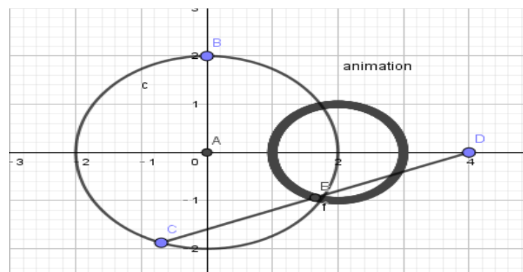
Figure-1. The trajectory of the midpoint of a line connecting a point outside the circle and a moving point on the circle.
